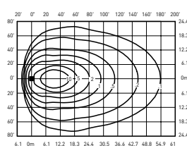
OSQL-C-40L-40K7-44-UL Mounting Height: 25' (7.6m) A.F.G., 60° Tilt Initial Delivered Lumens: 40,000 Initial FC at grade
